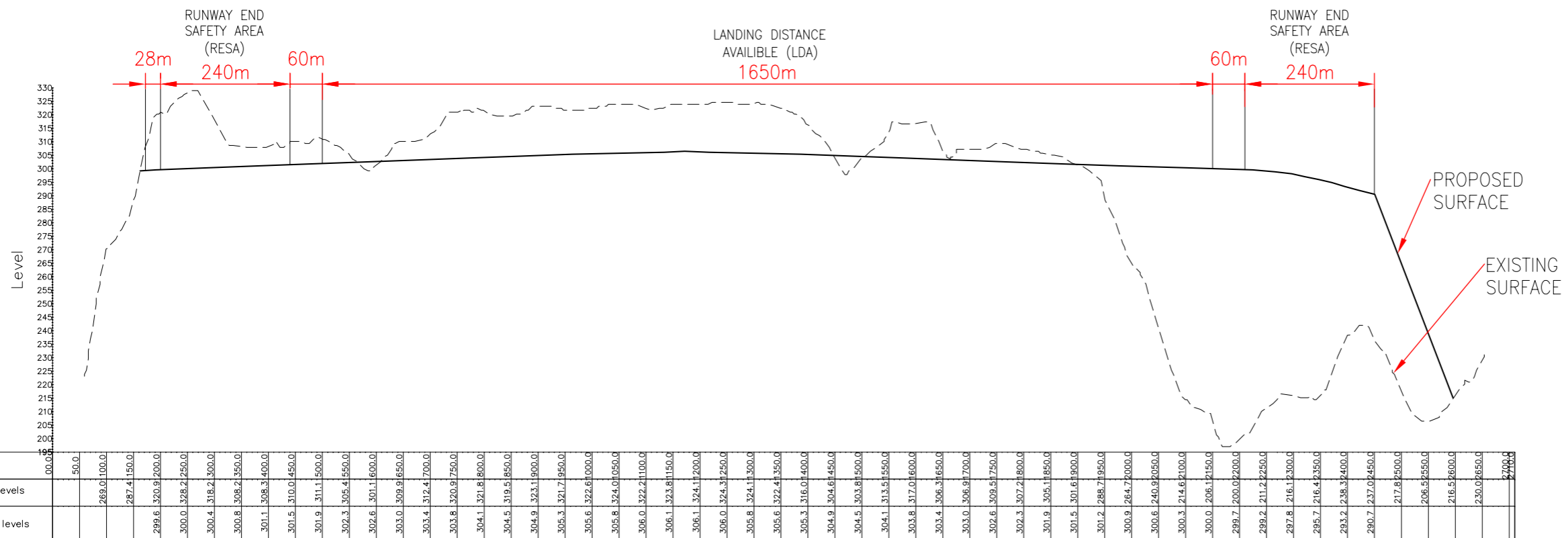
RUNWAY CENTRELINE SECTION Dimensions are in metres
