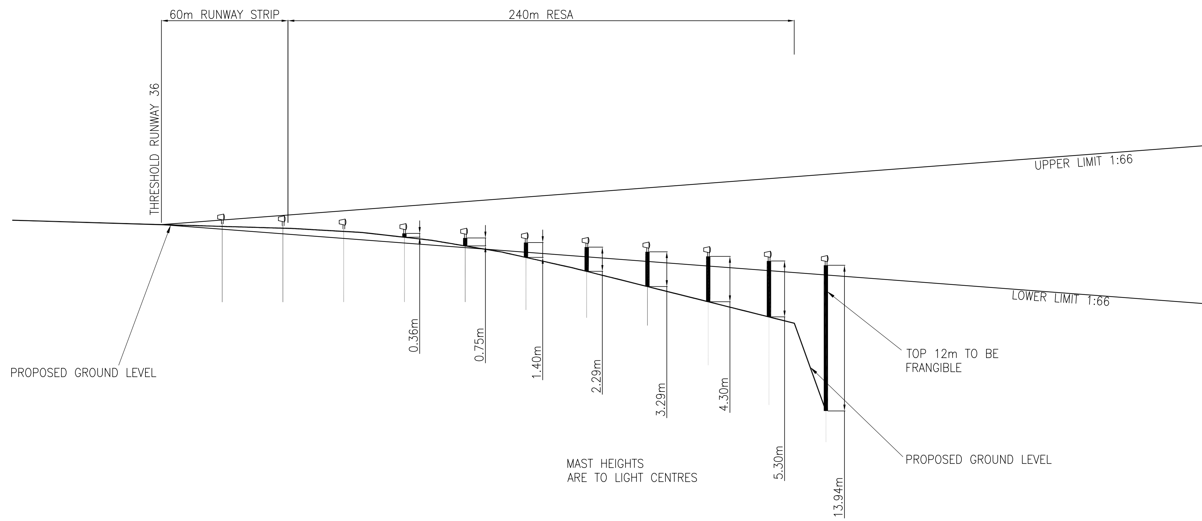
PROPOSED APPROACH LIGHTING PROFILE RUNWAY 36 Scale: V 1:200 H 1:1000
